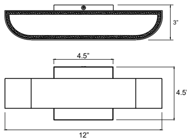
20046LEDDMG-SAT/FST Bi-Directional Outdoor LED Wall Mount Satin Finish Frosted Glass 12"W x 4.5"H x 3"Ext. 2 x 13.5 W SSL Dedicated LED (Included) 963 Delivered Lumens 3000K, 90 CRI, 120v Dimmable Wet Location UL (US/Canada) Listed ADA, JA8-2016/Title 24 Listed, Marine Grade
