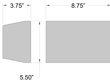
20019LEDDMG-SAT Bi-Directional Outdoor LED Wall Mount Satin Finish 8.75\"W x 5.5\"H x 3.75\"Ext. 2 x 10 W SSL Dedicated LED (Included) 911 Delivered Lumens 3000K, 90 CRI, 120v Dimmable Wet Location ETL (US/Canada) Listed ADA, JA8-2016/Title 24 Listed, Marine Grade
