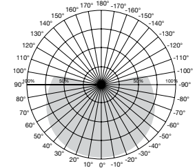
Beam Angle: 108°
