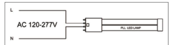
Wiring diagram
