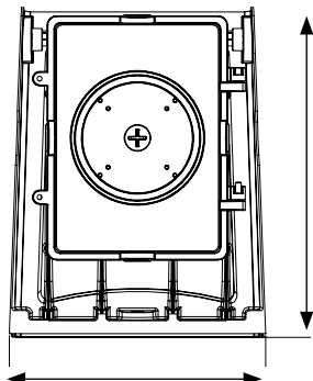
65-677, 65-678 3 7/8" (98.1±1mm) 65-679, 65-680 8 1/2" (216.1±1mm)
