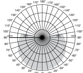
Beam Profile
