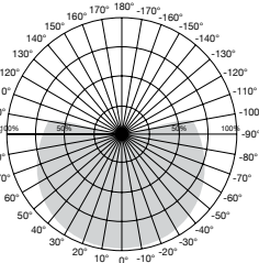
Beam Profile
