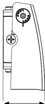
65-677, 65-678 3 7/8" (98.1±1mm) 65-679, 65-680 4 7/8" (112.1±1mm)
