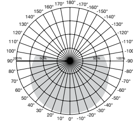
Beam Angle: 108°
