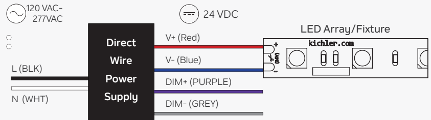
Typical Application and Wiring Diagram
