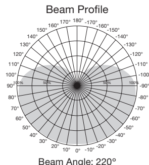
Beam Angle: 220°
