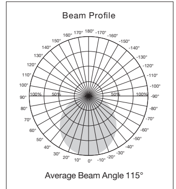
Beam Profile for Non-dimmable LED Low Bay Lamp 80W 120V-277V Ex39
