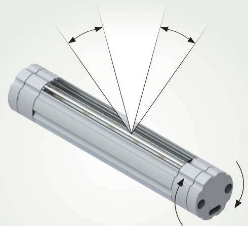
Rotate End Cap to adjust light spread when used with Accessory Beam Adjusting Insert and Beam Adjusting End Caps.
