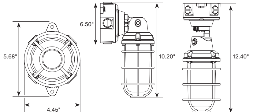
Fixture adjusts 90°
